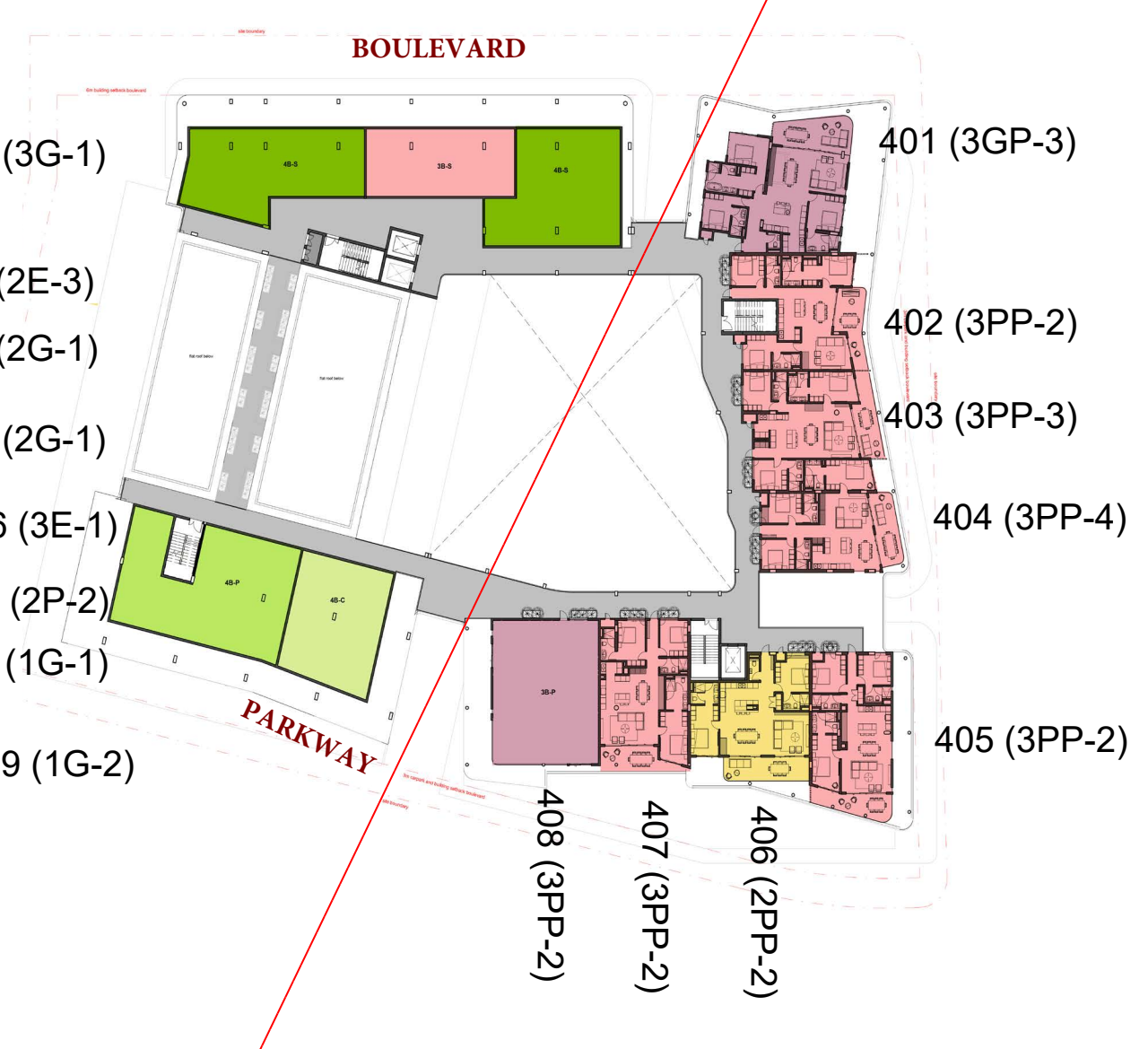
fourth floor
